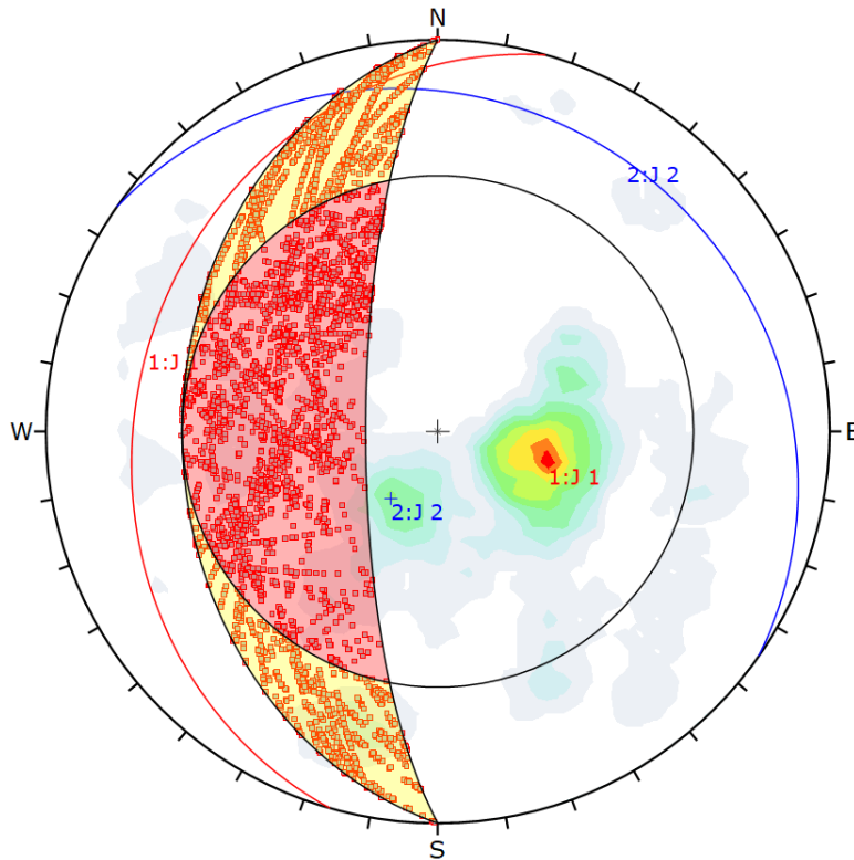
Figure 16-20 Kinematic analysis for the slope T3 showing 12% of probability for wedge rupture
