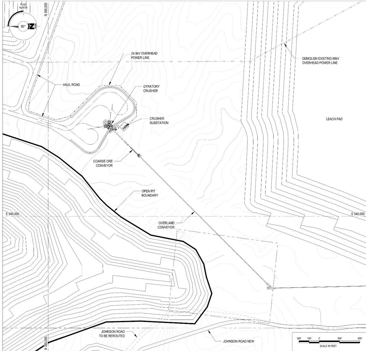
Source: M3, 2024 Figure 18-5: Primary Crusher Pad
