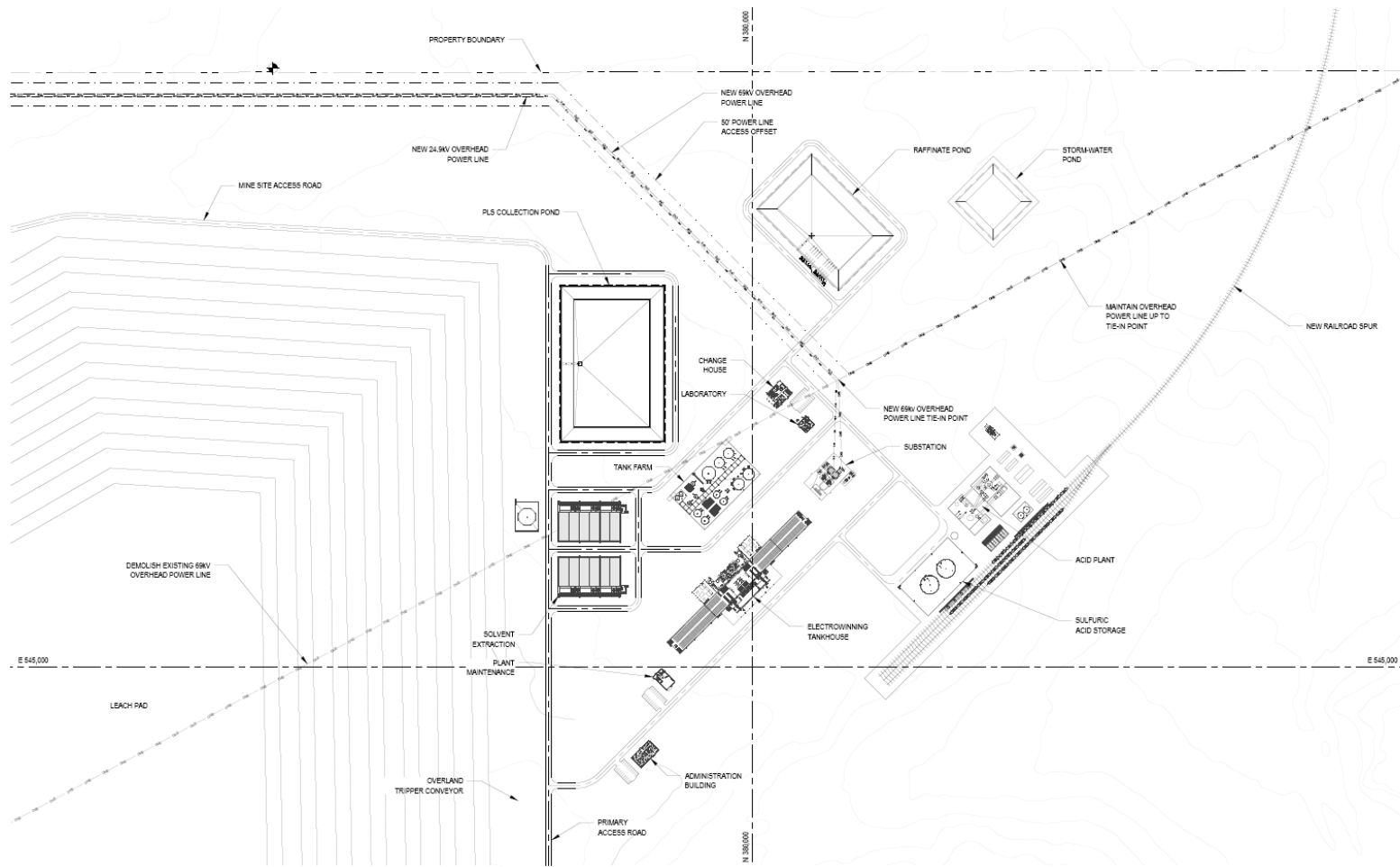
PROCESS PLANT SITE PLAN
