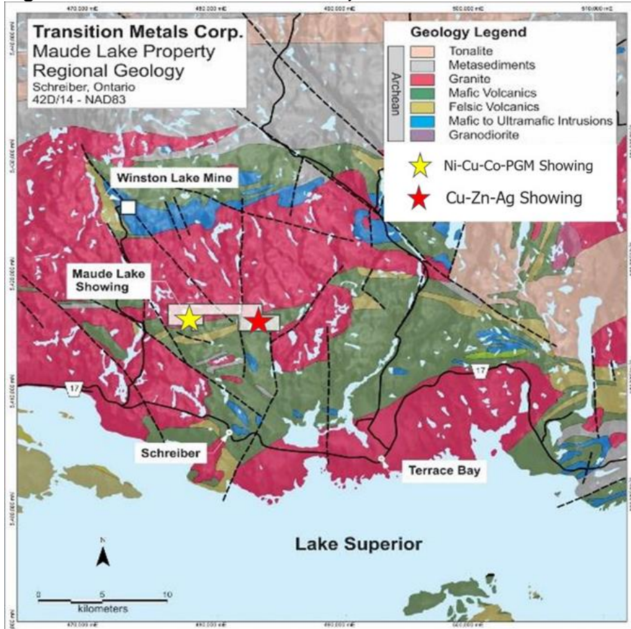
Figure 1: Location of the Maude Lake Project
