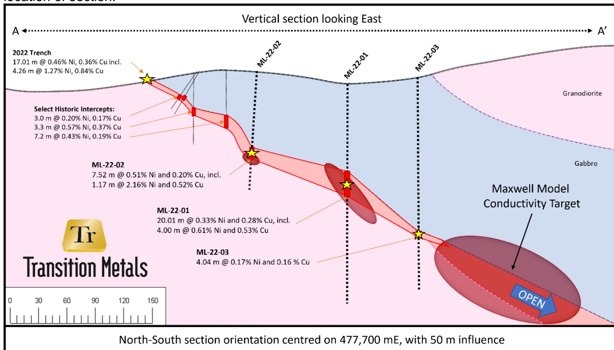
Figure 3: Composite vertical cross section with trench sampling and drilling results. See Figure 2 for location of section.
